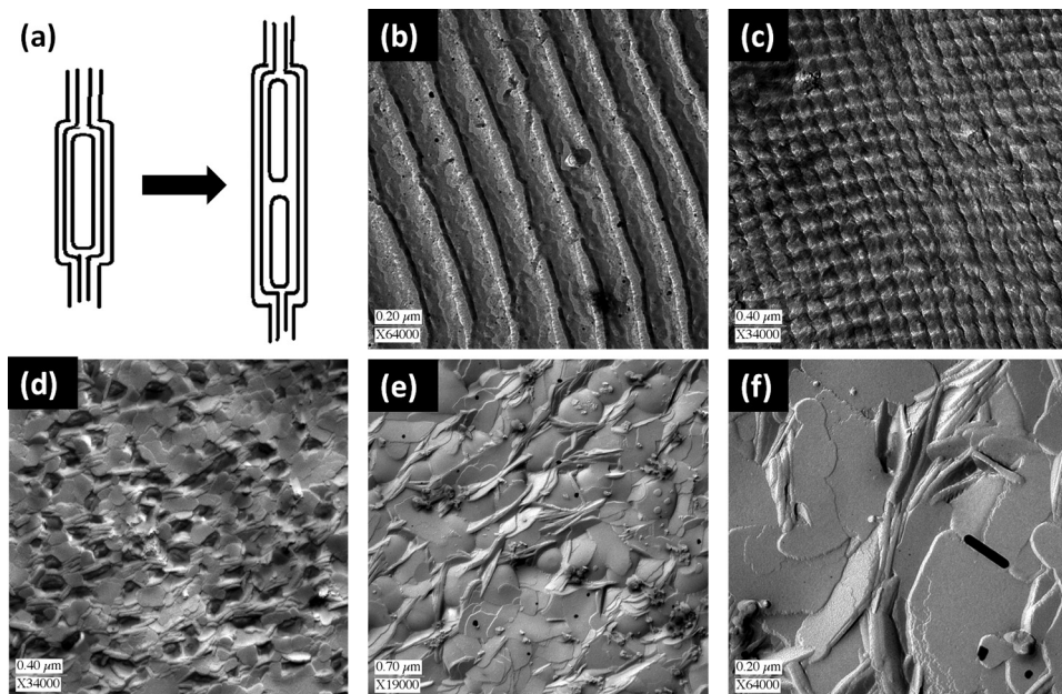
Figure 8. Spatial nanoscale structuring of nanorods dispersed in the 70% water, 25% CTAB, 5% BnOH hexagonal LC hosts. a) Rods in an aligned LC may form chains to reduce elastic energy due to the distortions at their ends. Freeze fracture transmission electron microscopy images of b) long rods forming chains and c) periodic structure in the plane orthogonal to the chains. d,e,f) different 3D networks of nanorods f) aligning along the domain walls between the nanoscale domains in the columnar hexagonal phase of the lyotropic LC.
